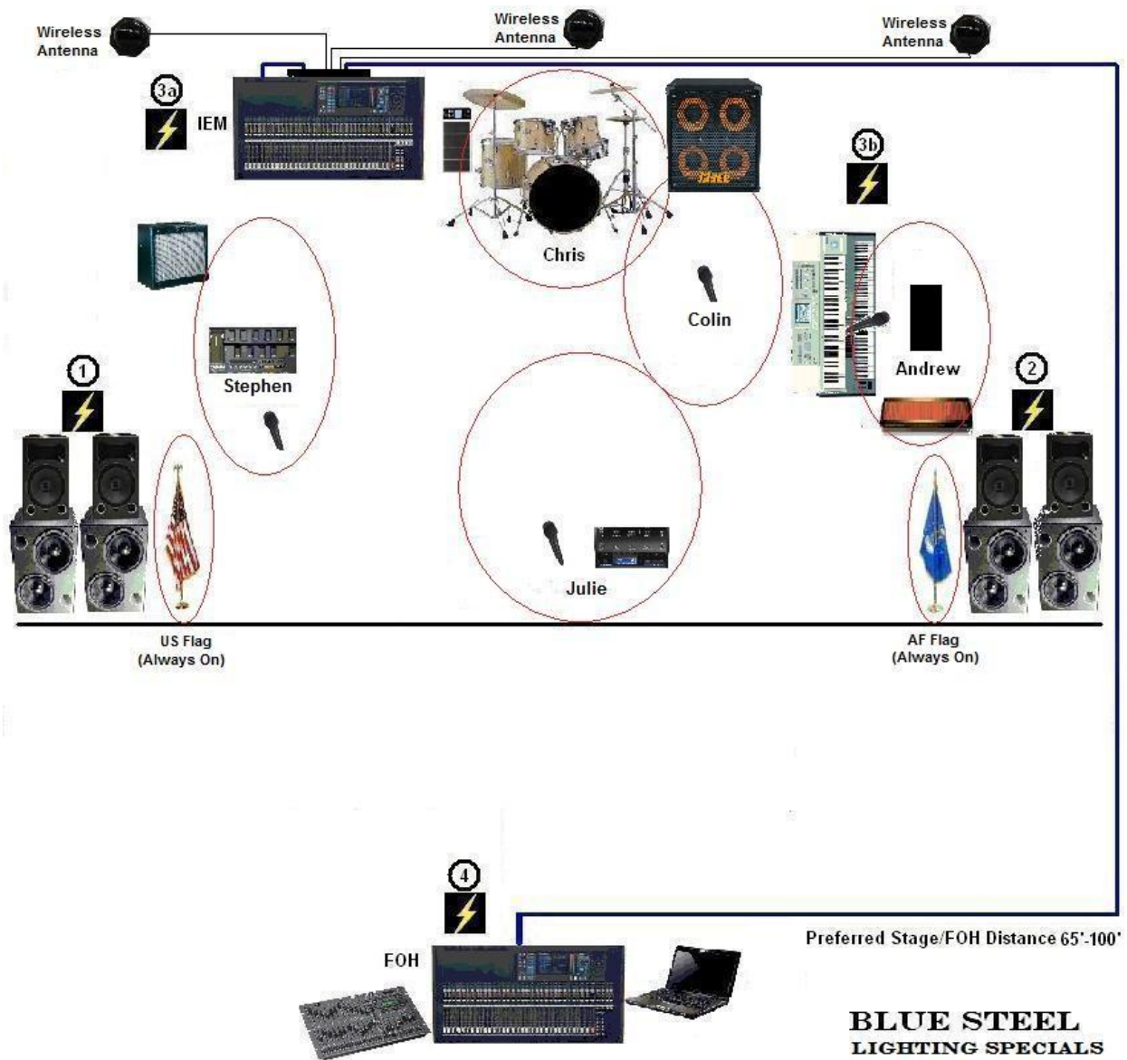
Figure 3. Lighting Specials
